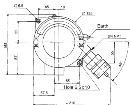
Explosion-proof case IP 66 - Type: RTPF EEx d IIC T6 - LCIE 01 ATEX 6071X
